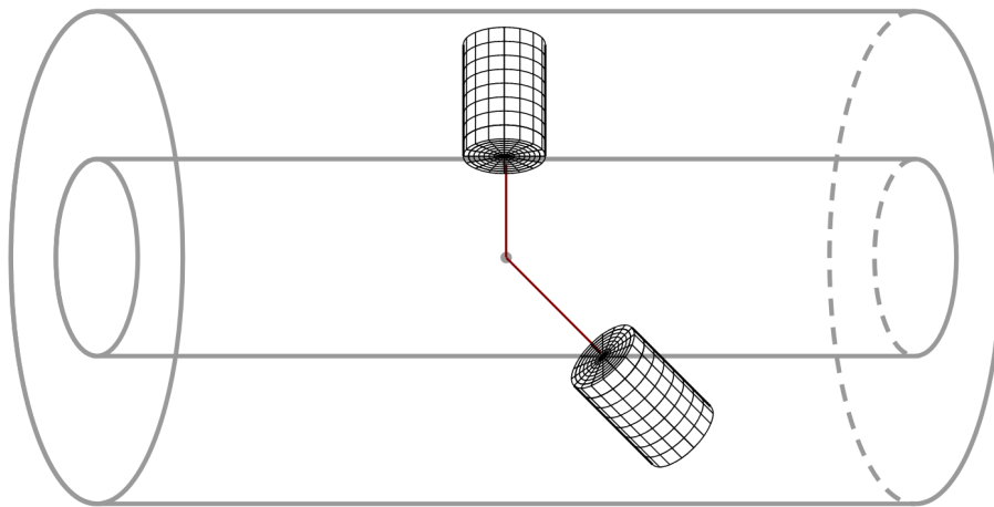
Fig. 11.1: Energy deposits are scored in cylindrical readout around particle momentum.
