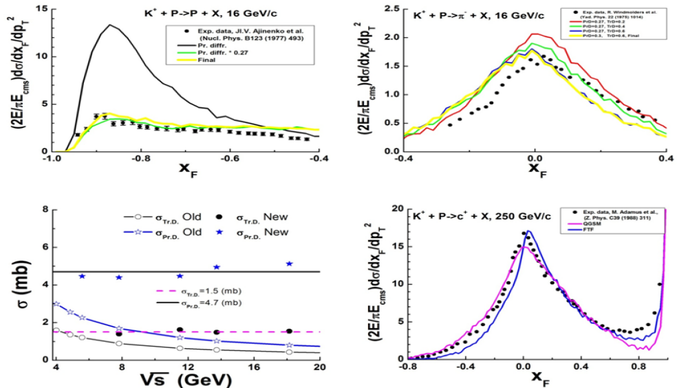
Fig. 24.13: Upper figures: inclusive spectra of protons and \pi^- -mesons in Kp^* -interactions. Points are experimental data* :cite:had-Ajinenko,had-Ajinenko2. Lines are FTF calculations. Bottom left figure: diffraction dissociation cross sections obtained by tuning (points), and their description (lines) by the expression for Kp in (24.4). Bottom right figure: x_F spectrum of positive charged particles in Kp -interactions at p_{lab} = 250 GeV/c. Points are experimental data [Whi74], lines are model calculations.
