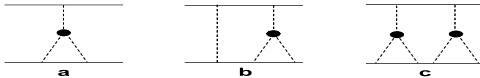
Fig. 24.17: Simplest enhanced diagrams of NN -scattering.
