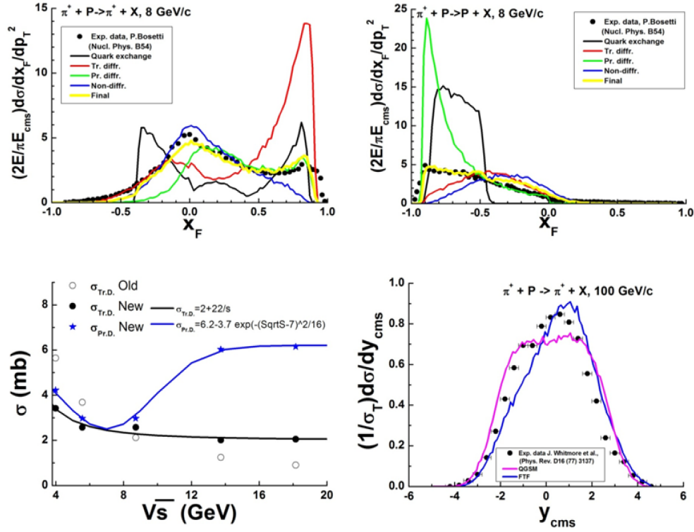
Fig. 24.12: Upper figures: inclusive spectra of protons and \pi^+ -mesons in \pi^+p -interactions. Points are experimental data [eal73b]. Lines represent the contributions of the various FTF processes calculated by assuming that the probability of each process is 100 %. Bottom left figure: diffraction dissociation cross sections obtained by tuning (points), and their description (lines) by the expression for \pi in (24.4). Bottom right figure: rapidity spectrum of \pi^+ -mesons in \pi^+p -interactions at p_{lab} = 100 GeV/c. Points are experimental data [Whi74].
