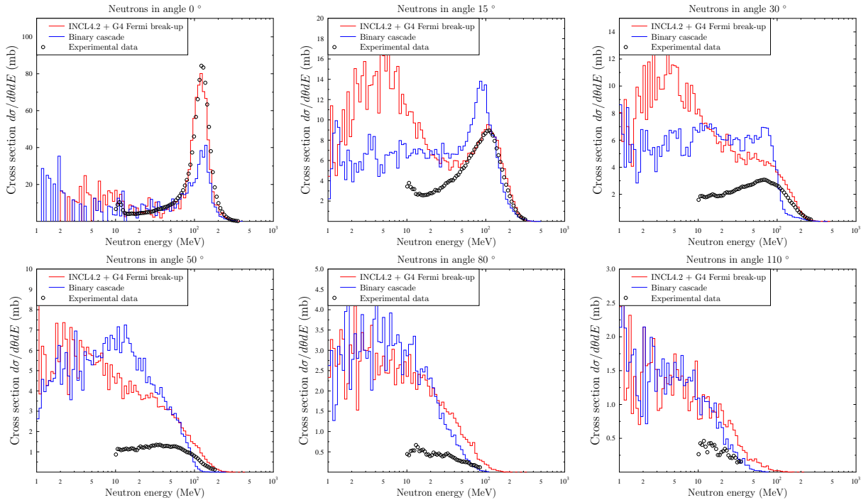
Fig. 1 Double-differential neutron energy spectra for C + C at 135 MeV/nucleon. INCL4.2 with Geant4 Fermi break-up and Geant4 Binary cascade are compared against experimental data from reference 11 ).
