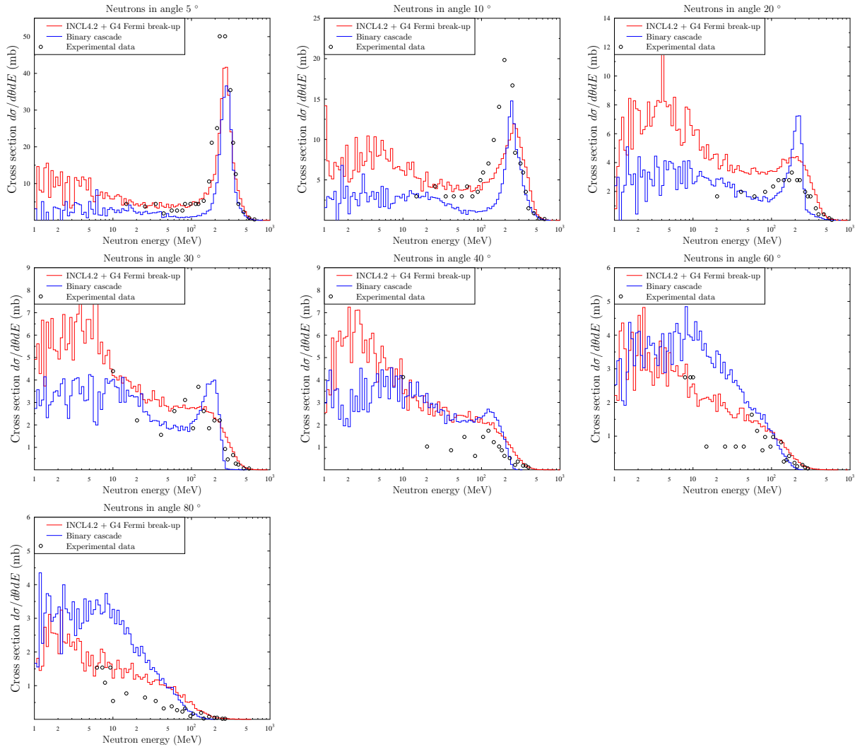
Fig. 2 Double-differential neutron energy spectra for C + C at 290 MeV/nucleon. INCL and Geant4 Binary cascade are compared against experimental data from reference 12) .
