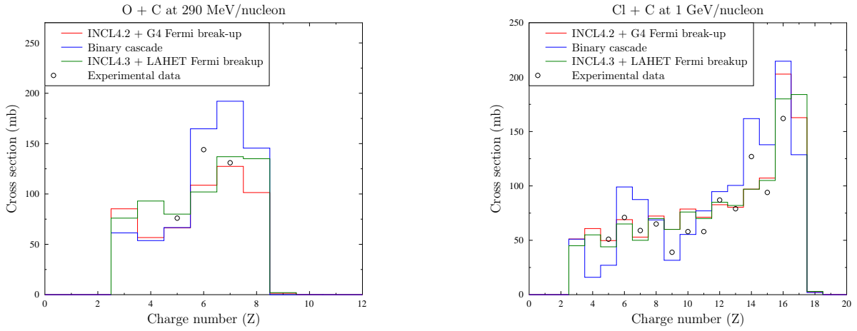
Fig. 3 Oxygen (left) and chlorine (right) fragmentation of INCL4.2 (C++) with Geant4 Fermi break-up for light fragments (mass 16 and below) and ABLA for heavier fragments, Binary cascade, and INCL4.3 (FORTRAN) compared against experimental data from references 13, 14 . For technical reasons all calculations are done using inverse kinematics.
